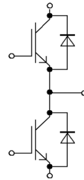
Equivalent Circuit Schematic
